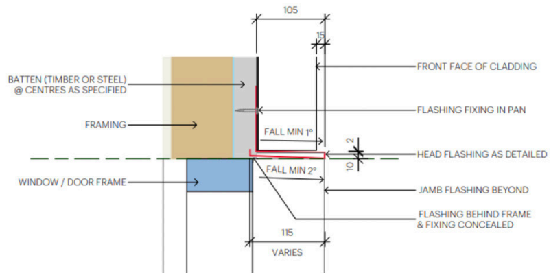
NINELINE™ Pleat | Window Head & Sill Flashings
