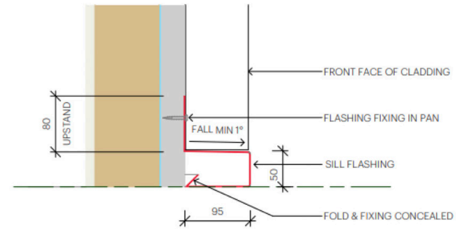
NINELINE™ Pleat | Toe Flashing
