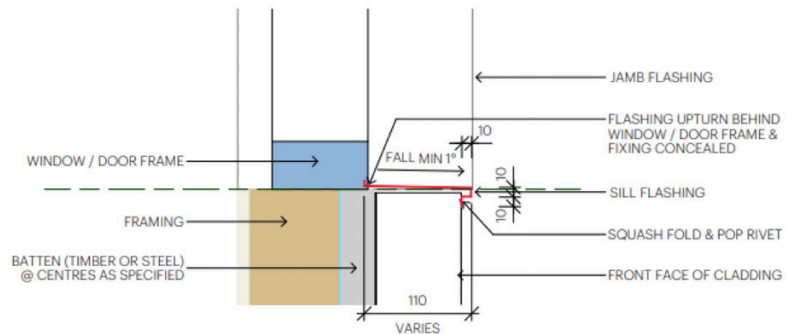
NINELINE™ Pleat | Window Head & Sill Flashings
