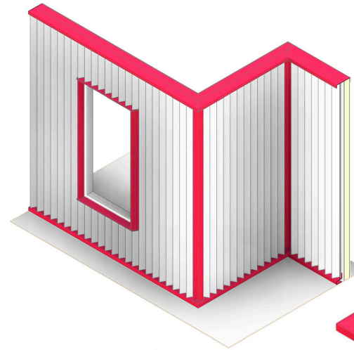
NINELINE™ Pleat | Assembly
