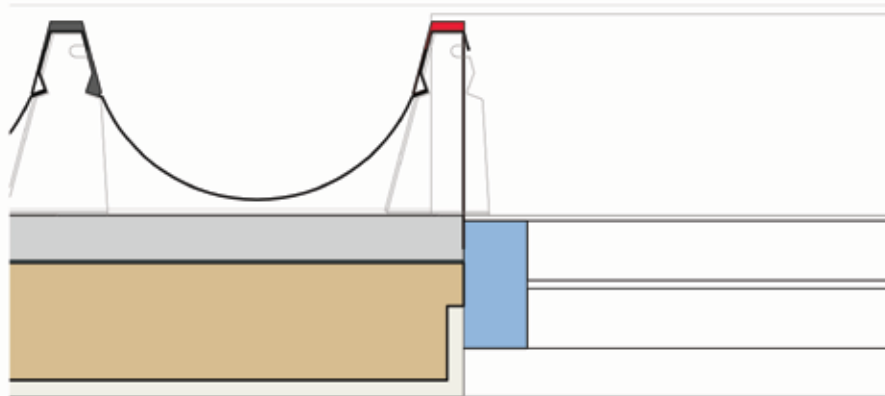
NINELINE™ Flute | Window Jamb 1
