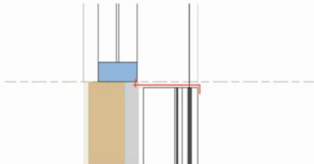
NINELINE™ Flute | Window Head & Sill Flashings
