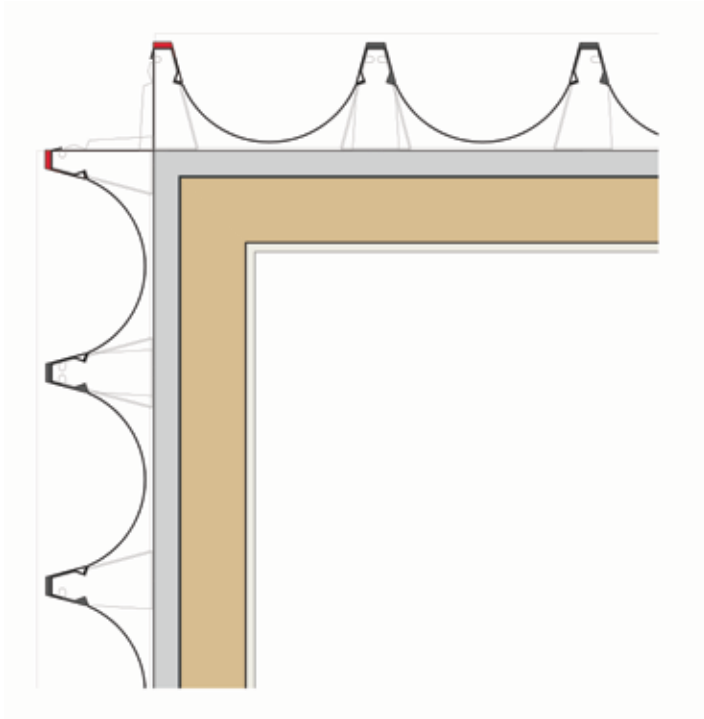
NINELINE™ Flute | Ext Corner
