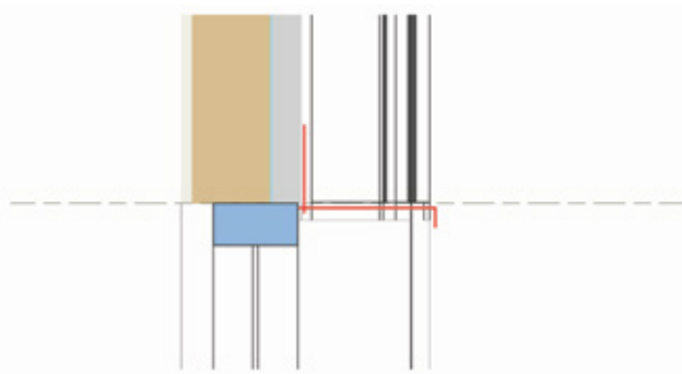
NINELINE™ Flute | Window Head & Sill Flashings
