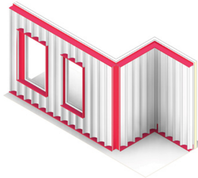
NINELINE™ Flute | Assembly
