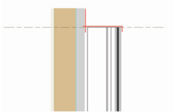
NINELINE™ Flute | Parapet Flashing
