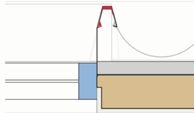
NINELINE™ Flute | Window Jamb 2
