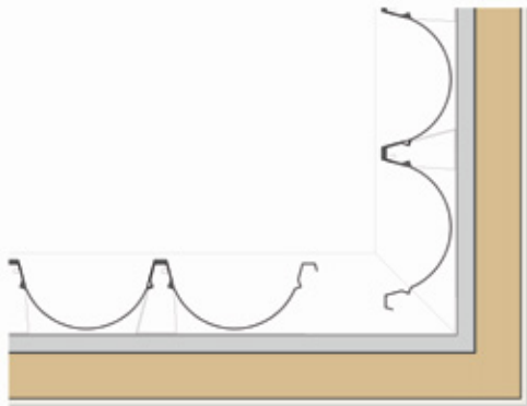
NINELINE™ Flute | Int Corner Typ
