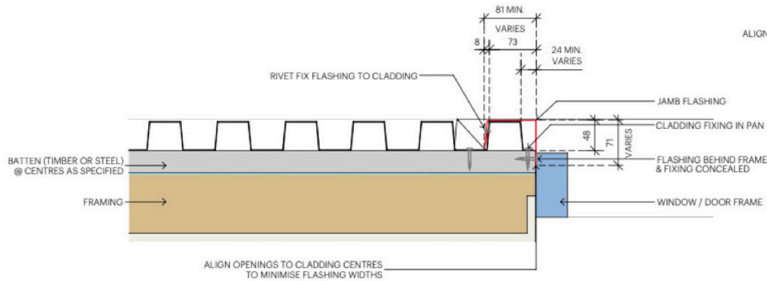
NINELINE™ Batten | Window Jamb 1
