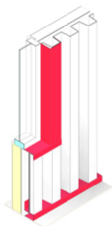
NINELINE™ Box | Window Jamb
