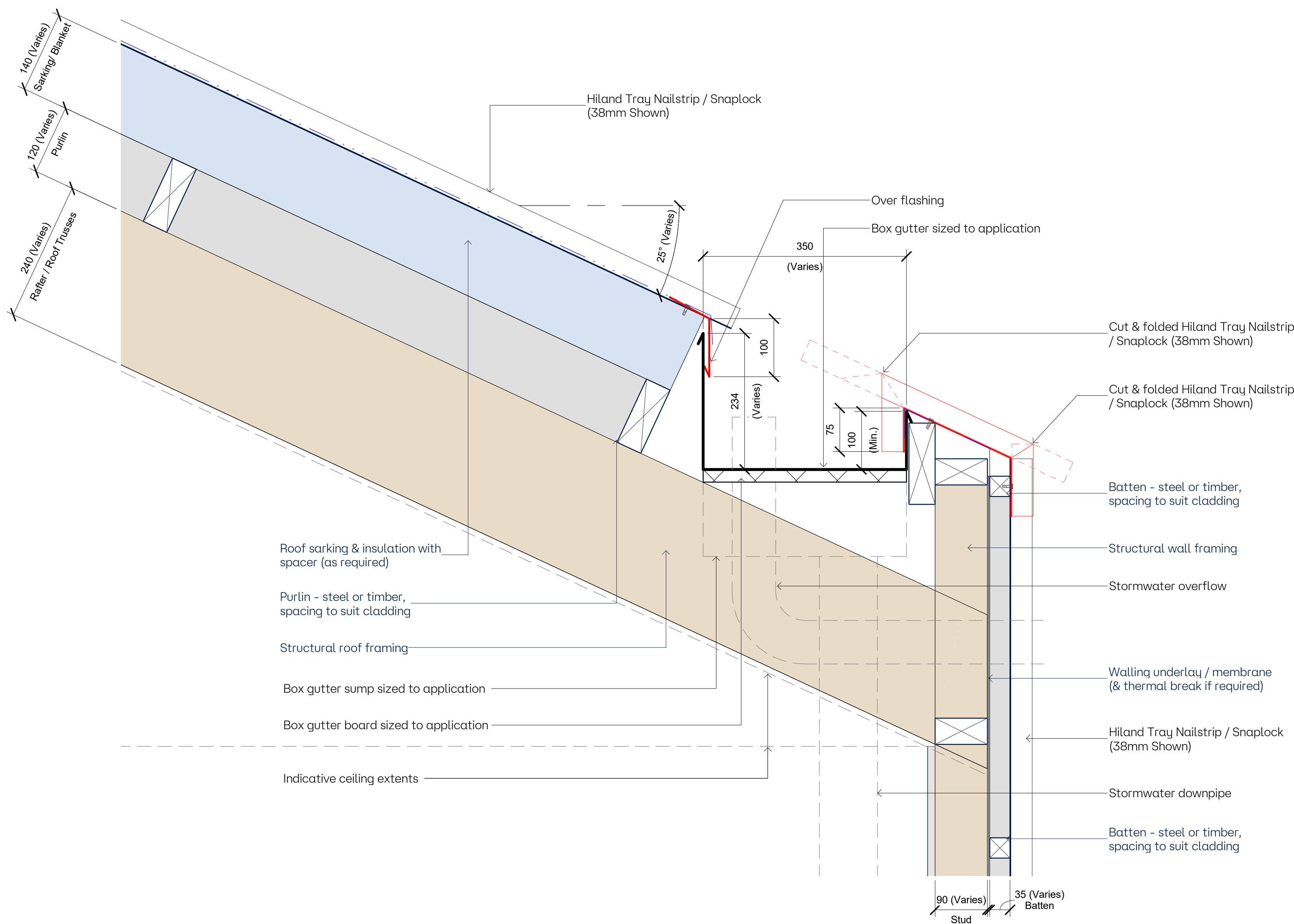
1 Hiland Nailstrip / Snaplock Mansard 1 : 5
